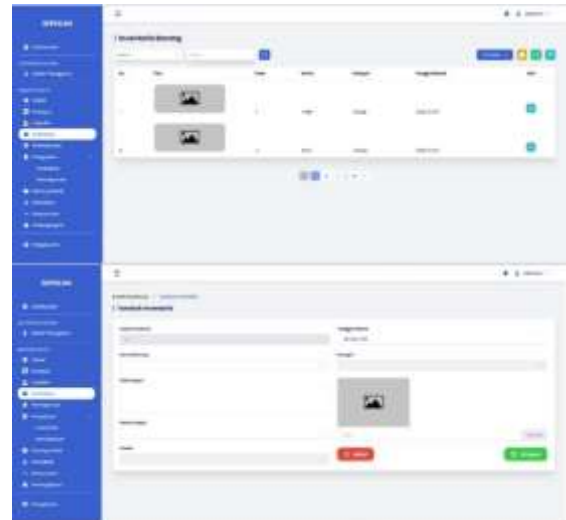
Gambar 8. Menu Inventaris
