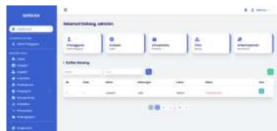
Gambar 3. Dashboard Sepekan
