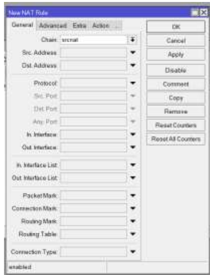
Gambar 18 Tampilan Firewall NAT
