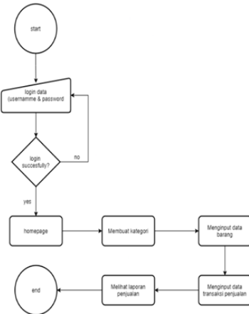
Gambar 1 Rancangan Flowchart
