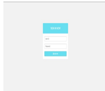
Gambar 3 Form Login
