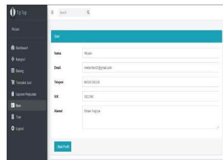
Gambar 9 Tampilan User
