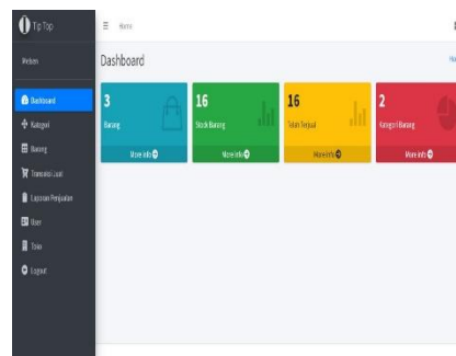
Gambar 4 Dashboard
