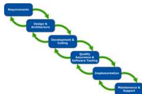
Gambar 1 Model Waterfall
